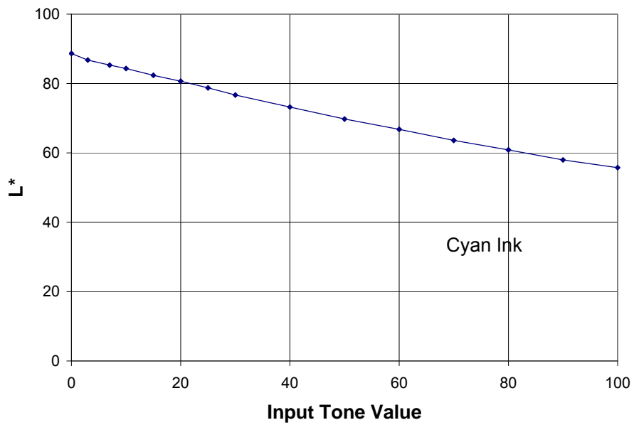
Figure A.3 — L* vs. input tone value for cyan scale
